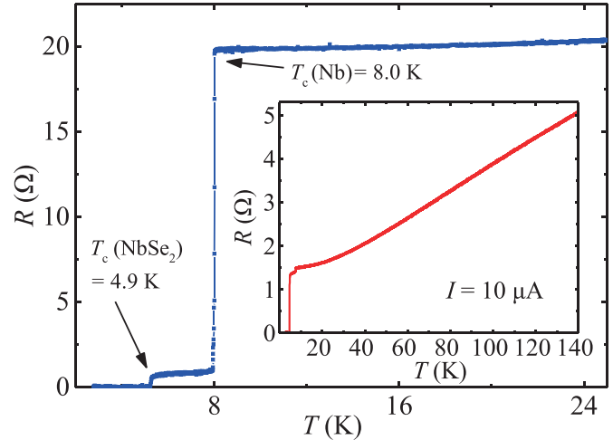
Figure 2. Temperature dependence of the sample resistance, measured across junction 3. The transition temperatures of Nb and NbSe 2 are indicated. The inset shows the resistance of the NbSe 2 flake for temperatures below 140 K. For both measurements the bias current is 10 \mu\text{A} .
