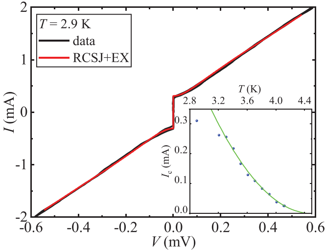
Figure 3. IVC of junction 3, measured at T = 2.9 K (black line). The red line is a fit based on the RCSJ+EX model with a Stewart–McCumber parameter \beta_c = 0.1 , i_{ex} = 0.65 and \alpha = 0.7 . The inset shows the temperature dependence of the junction critical current. The green line is the parabolic function I_c \propto (1 - T/4.5 \text{ K})^2 .
